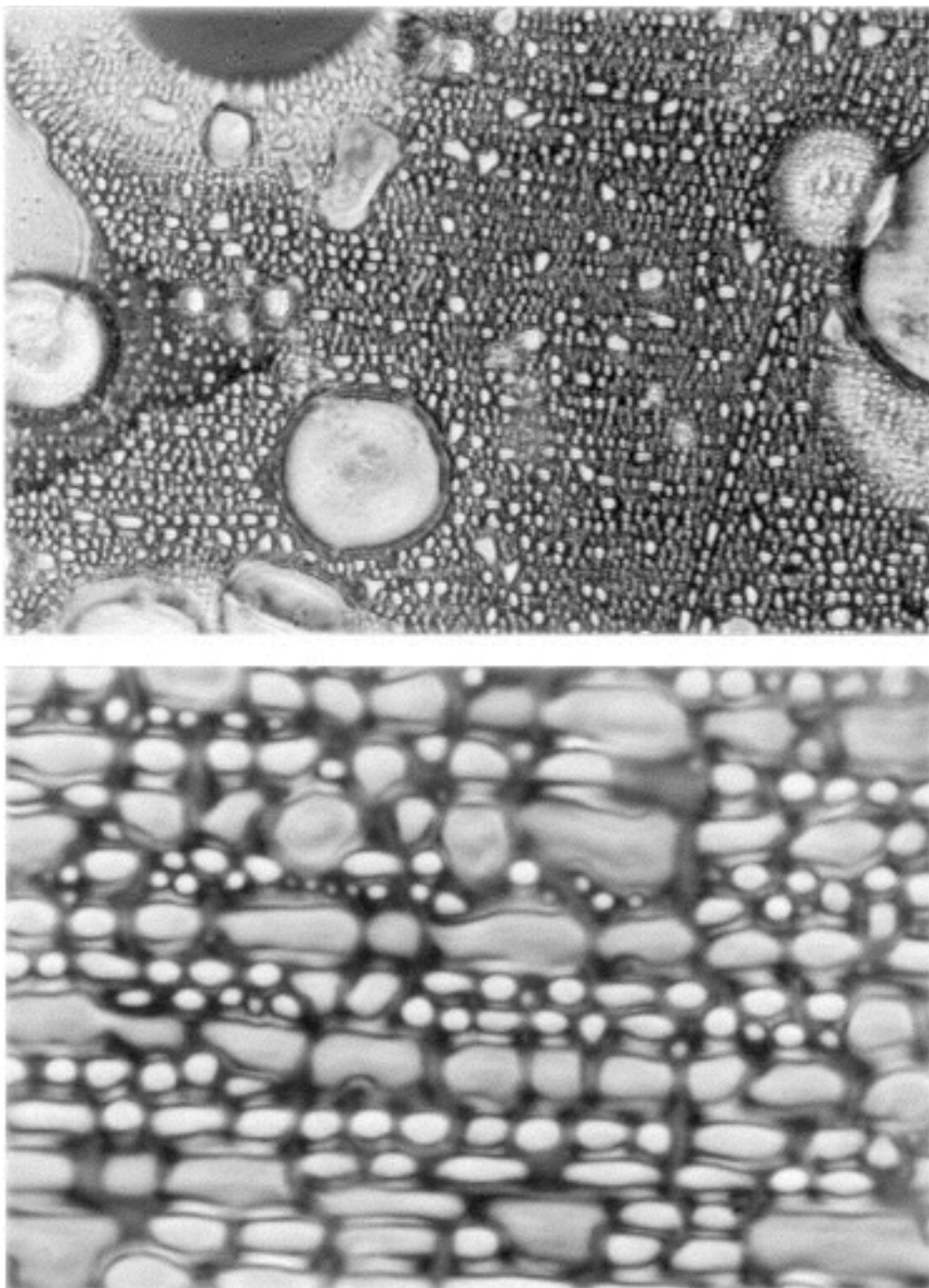
Figure 4.15. The top picture depicts under a 10X magnification a liquid magnecule composed of a bond between fragrance oil and water, the lower picture showing its 100X enlarged view.
